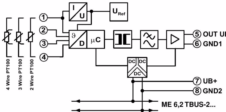
Figure 4 Block diagram
